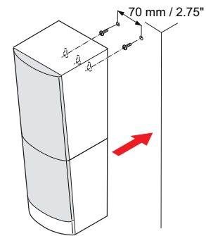
Fig. 2: Wall mounting
