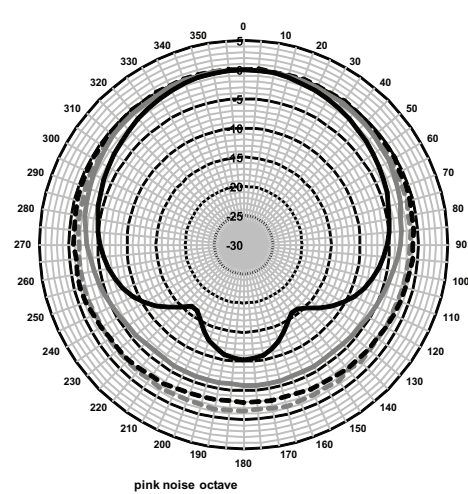
Fig. 8: Polar diagram (measured with pink noise)
