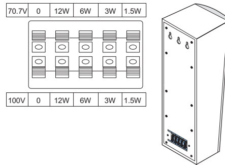
Fig. 1: Power setting
