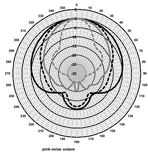
Fig. 7: Polar diagram (measured with pink noise)
