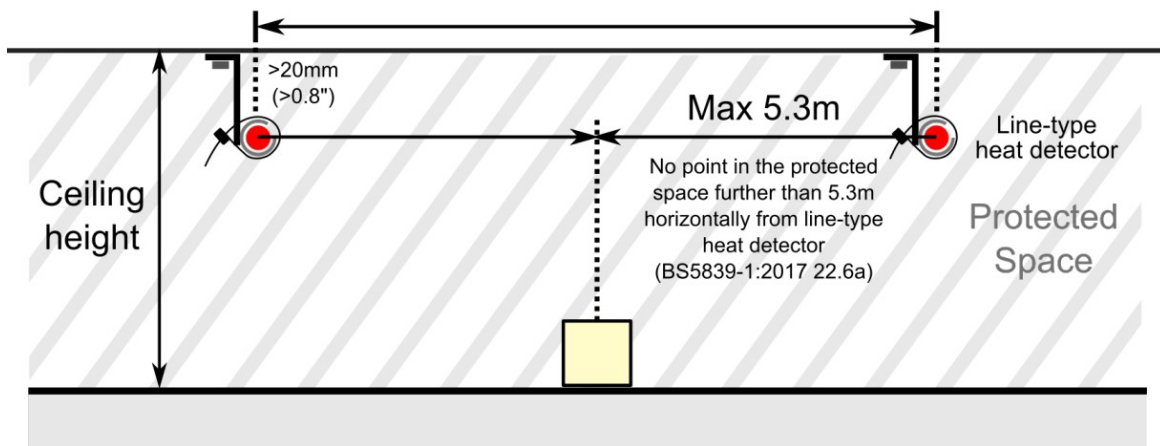
Fig. 5 Spacing requirements for Signaline FT-EN Linear Heat Detection cables
