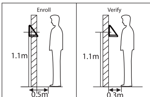
Non-identical distance
