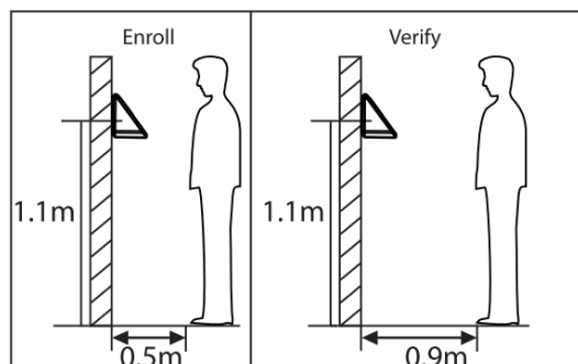
Non-identical distance
