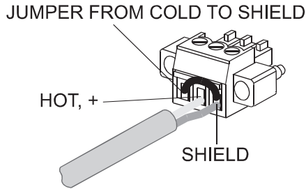
Figure 6.3: Unbalanced cabling
