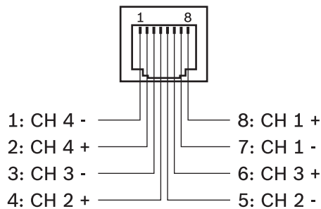
Figure 6.1: Pin assignment of LINE IN 1-4 socket
