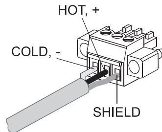
Figure 6.2: Balanced cabling
