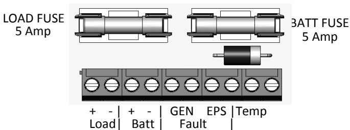
Figure 4 – Terminal labels
