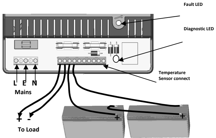
Figure 3 – Connections
